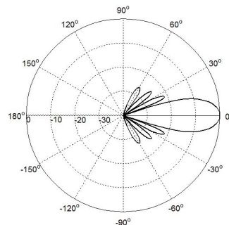
Elevation(High band)
