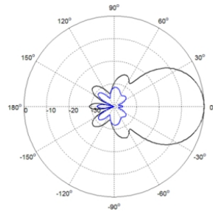
Azimuth(High Band)
