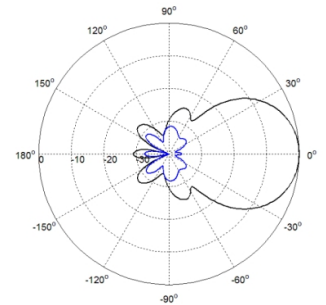
Elevation(High Band)
