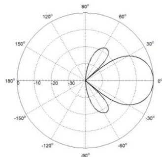
Elevation(Low band)
