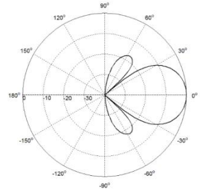
Elevation(High band)
