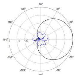
Azimuth(1695-2690MHz)
