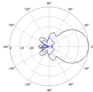
Elevation(Low Band)
