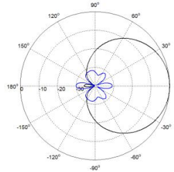
Azimuth(1710-2690MHz)
