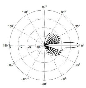
Elevation(High Band)
