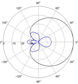
Azimuth(Low band)
