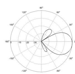
Elevation(1695-2690MHz)
