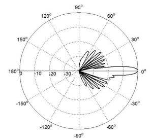
Elevation(High Band)
