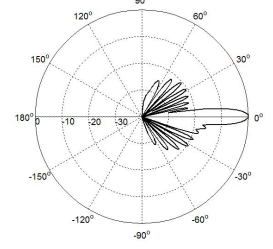
Elevation(1710-2690MHz)
