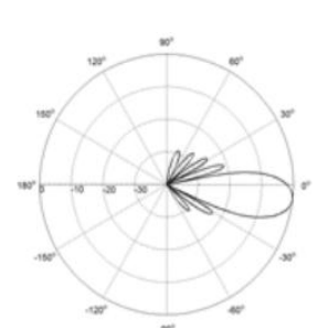
Elevation(High band)
