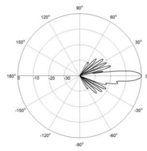
Elevation(Low Band)
