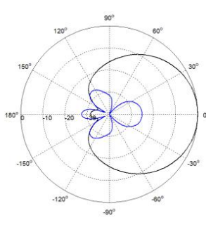
Azimuth(Low band)
