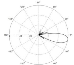
Elevation(1695-2690MHz)
