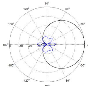
Azimuth(High band)
