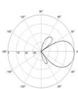
Elevation(Low band)
