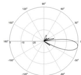
Elevation(1695-2690MHz)
