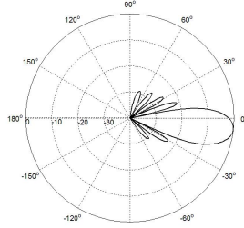
Elevation(698-960MHz)
