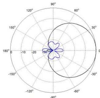
Azimuth(High band)
